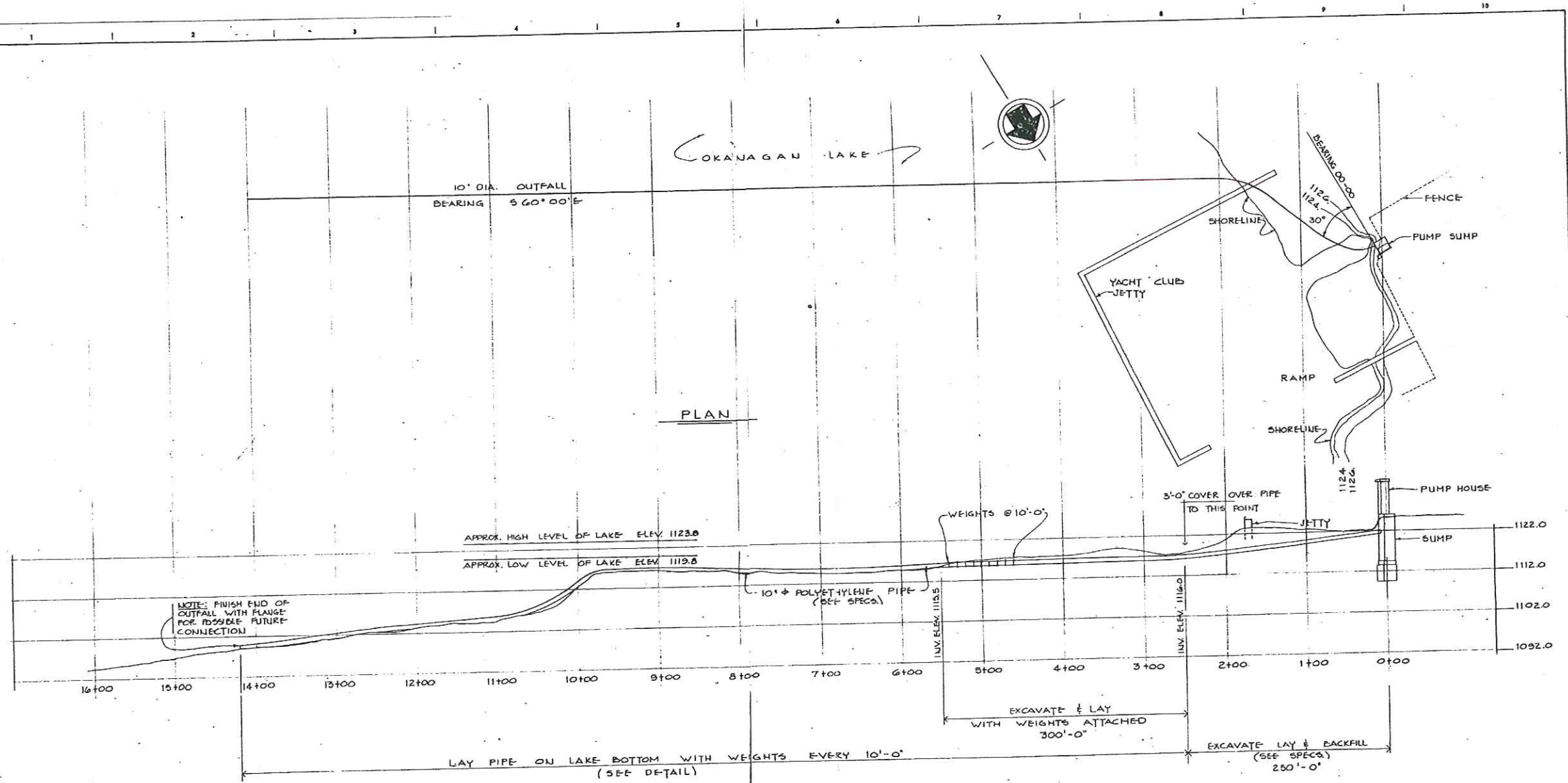
OUTFALL PROFILE
