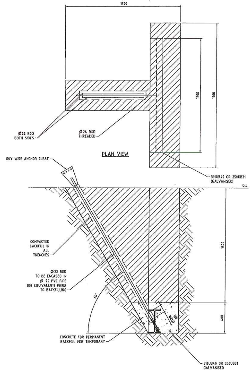
TYPICAL GUY ANCHOR FOOTING DETAIL
