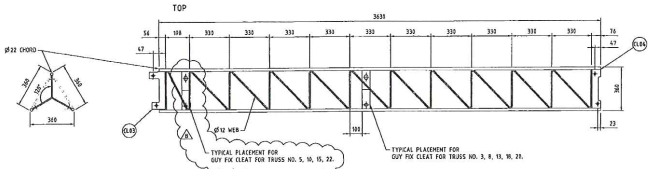
3630 TYPICAL MAST SECTION
