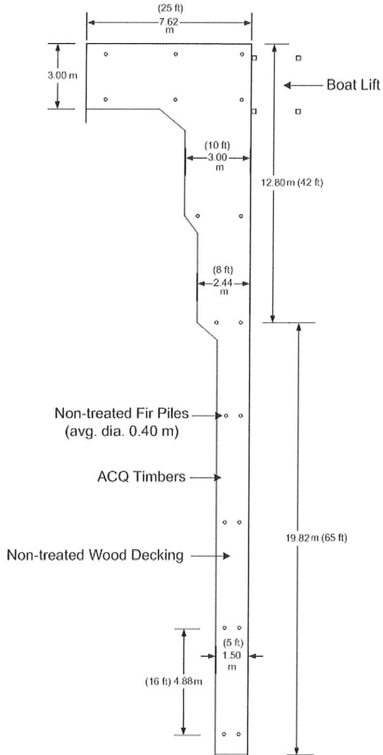
Figure 2. Plan view of proposed dock at 8997 Peters Road on Okanagan Lake.
