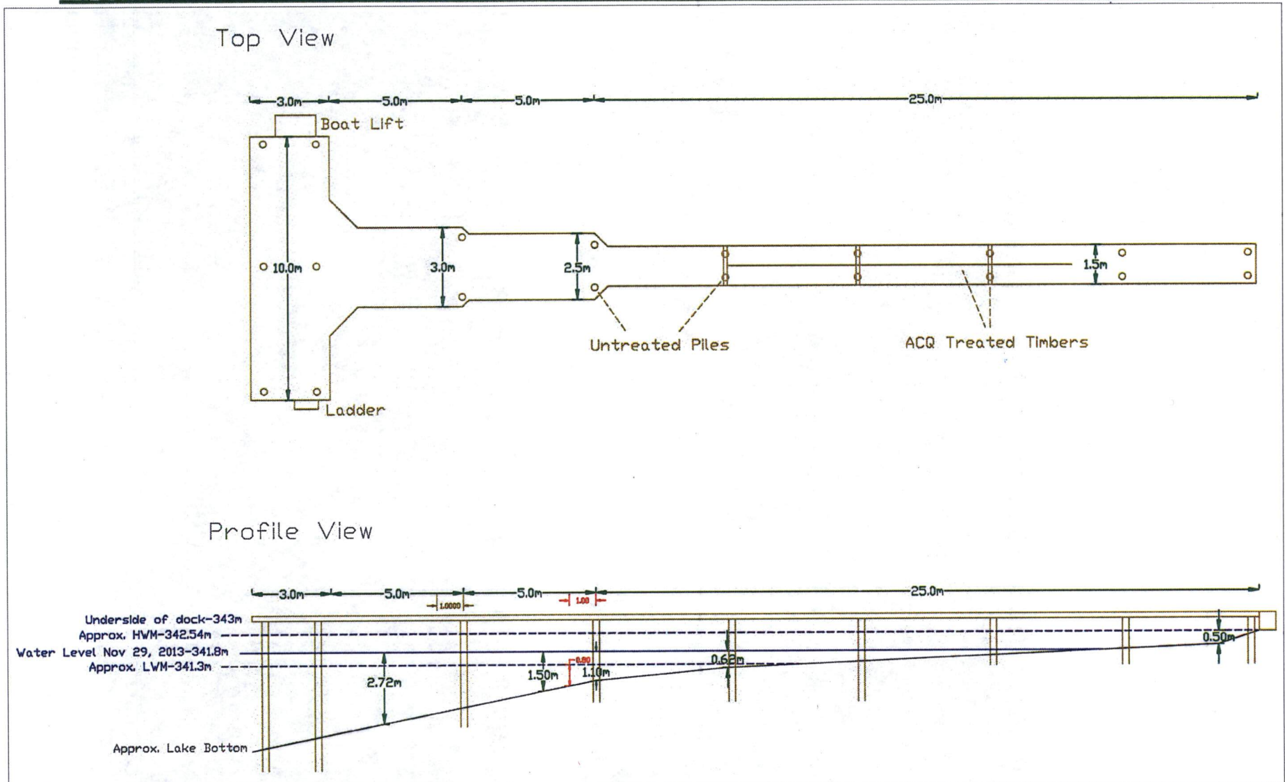
Figure 3. Sketch plan showing top and profile views of proposed dock structure.
