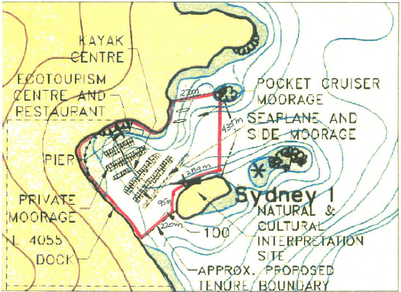
Figure 3.1. Overall proposed site plan.
