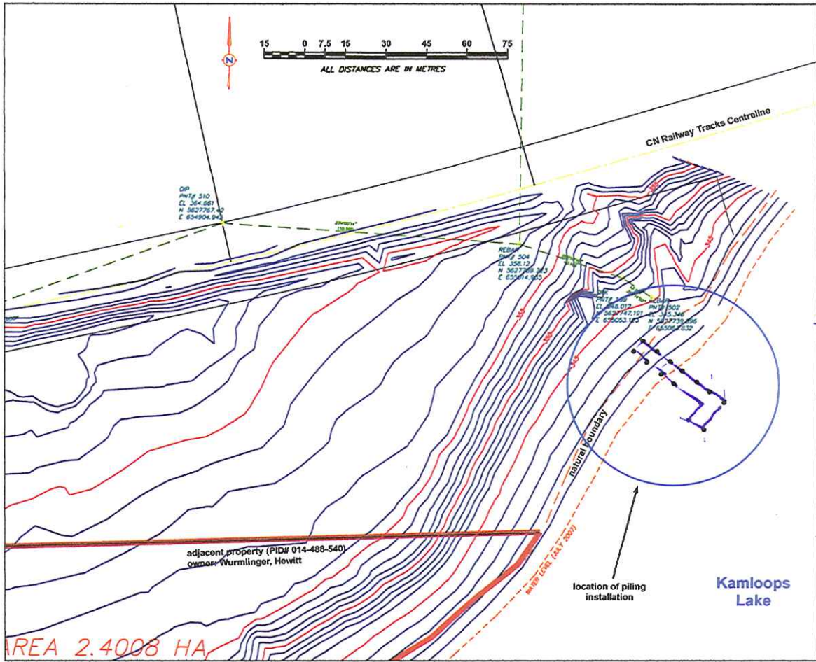
Figure 3. Survey plan of the property, illustrating the proposed location of the dock installation and adjacent property location. Each black dot indicates a single steel piling. Scale 1:2000.
