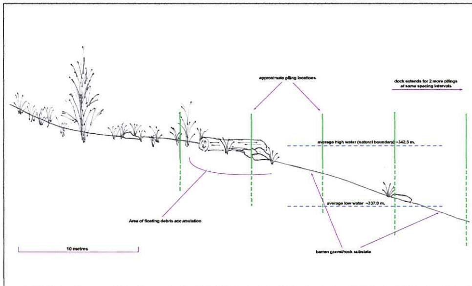
Figure 4. Cross-section of proposed location for dock. Scale is approximate.
